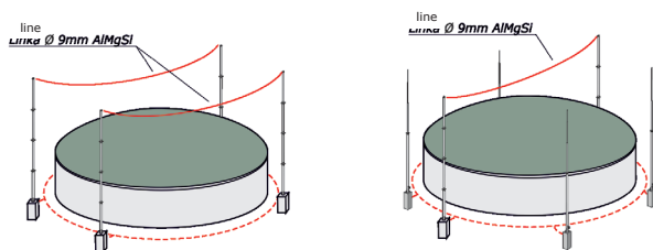
Facility protection using masts AH070001W in a system with free-standing masts.
